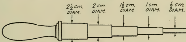
FIG. 200.—Mandrels for Testing the Pliability of Prepared Roofings.
